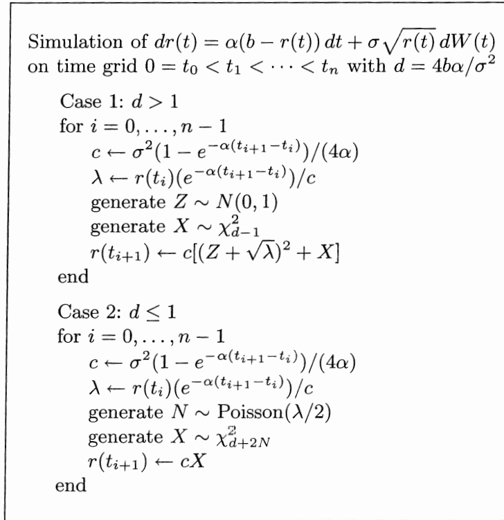
Fig. 3.5. Simulation of square-root diffusion (3.62) by sampling from the transition density.
